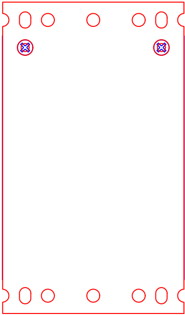
MPS-D0
